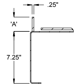
1/4" WELD ON FLAT BAR
