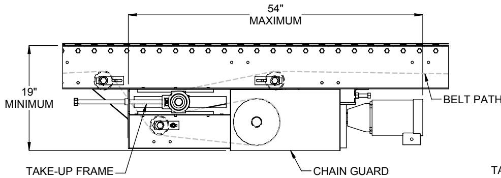
CENTER DRIVE OPTION
