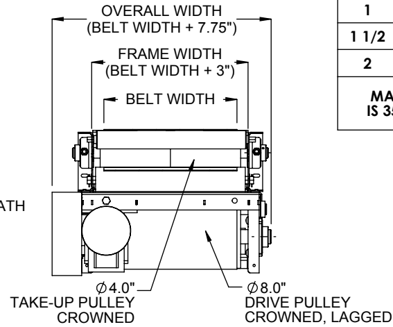
CENTER DRIVE END VIEW
