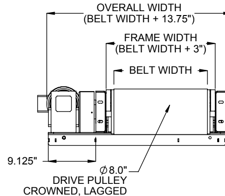
SIDE DRIVE END VIEW
