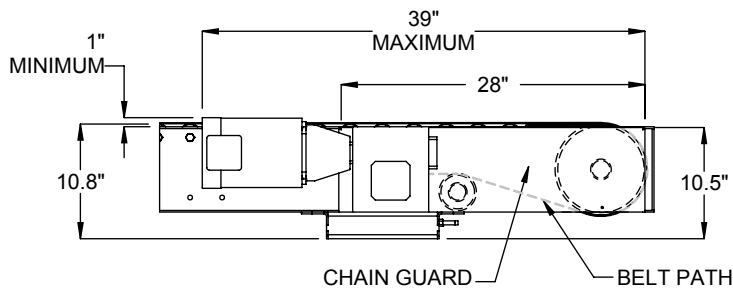
SIDE DRIVE OPTION
