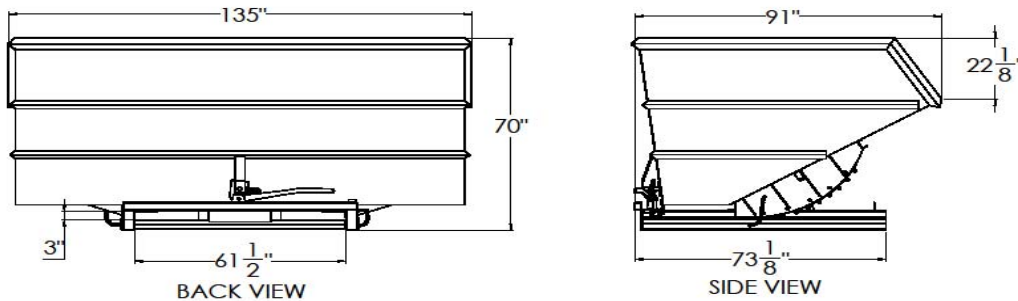
BEHEMOTH 5T-1/4-EL-2700
