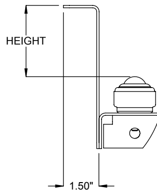
GUARDRAIL
