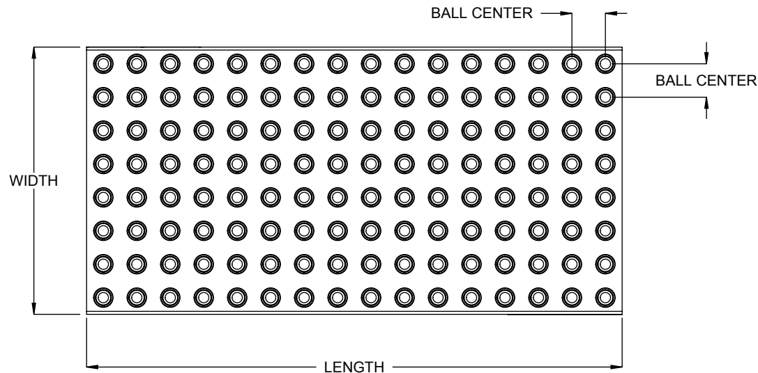
BALL TRANSFER TABLE STYLE A, STRAIGHT BALL PATTERN
