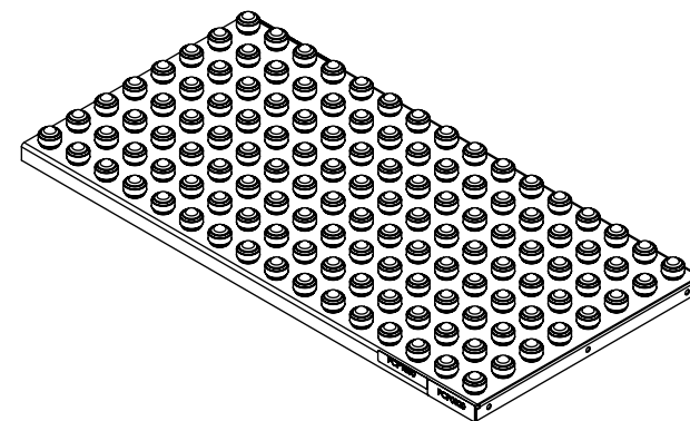
BALL TRANSFER TABLE STYLE A STRAIGHT BALL PATTERN
