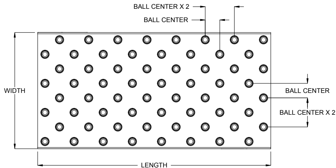
BALL TRANSFER TABLE STYLE A, STAGGERED BALL PATTERN
