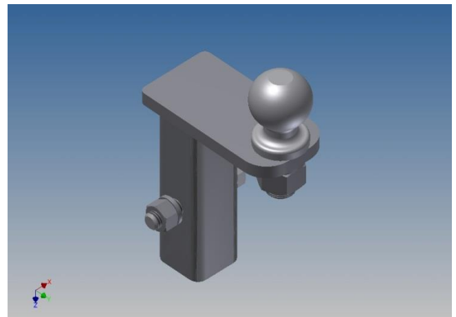
LM0401 (SA, Standard Ball Hitch Att.)
