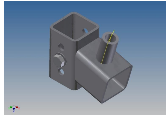
LM0453 (SA, Vertical Pin Lift Attachment)
