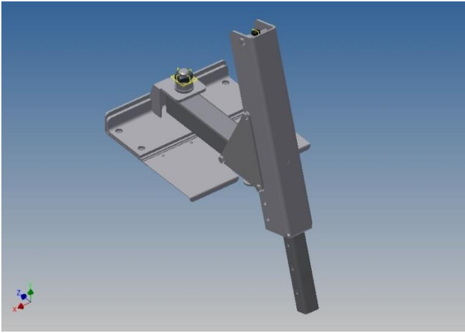
LM0329 (SA, 5th Wheel 2.0)
