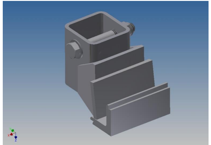
LM0386 (SA, Xtra 5th Wheel Hook)
