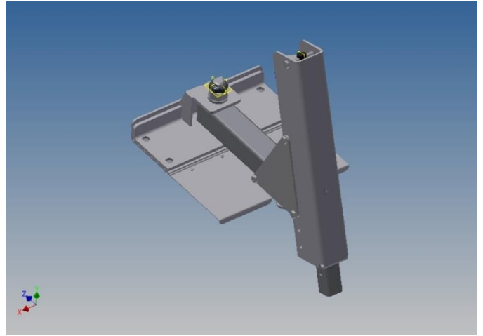
LM0452 (SA, Xtreme 5th Wheel)
